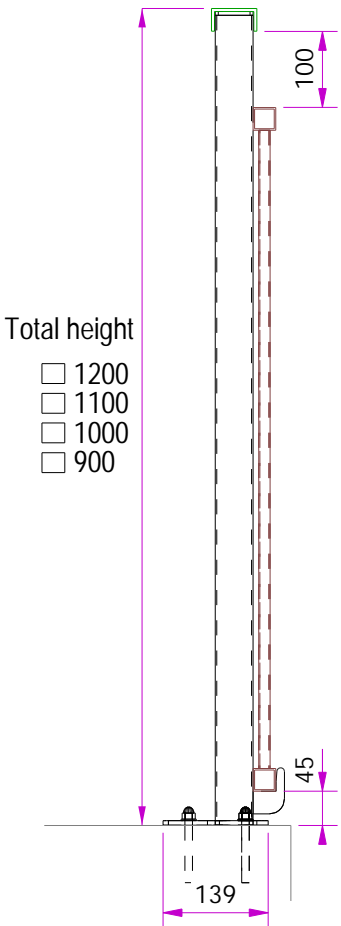
Side view 1:10
