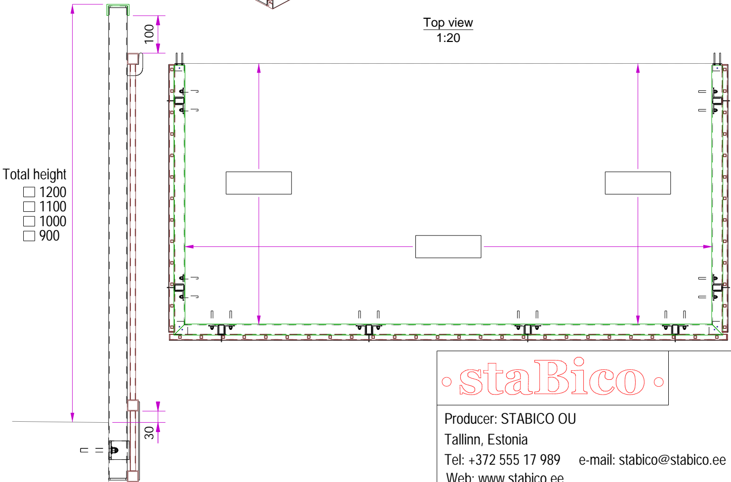
Side view 1:10
