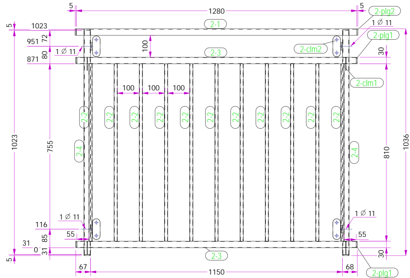
Front view 1:10
