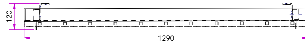
Top view 1:10
