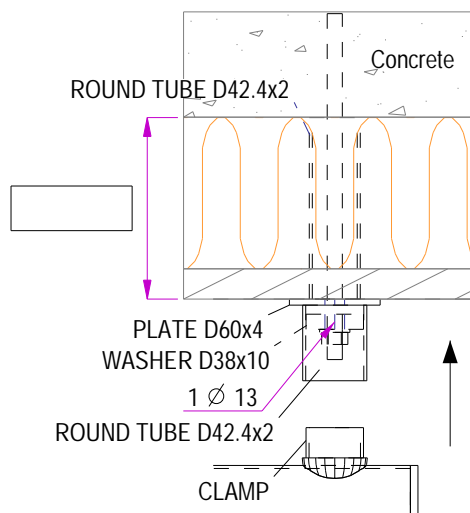
Detail 1 1:5
