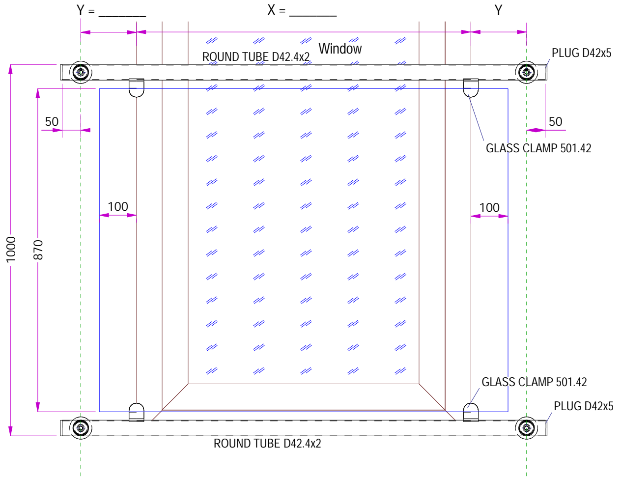
Top view 1:10
