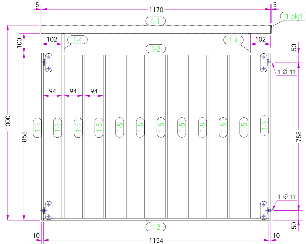
Front view 1:10
