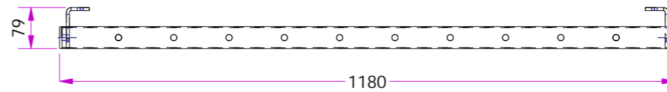
Top view 1:10
