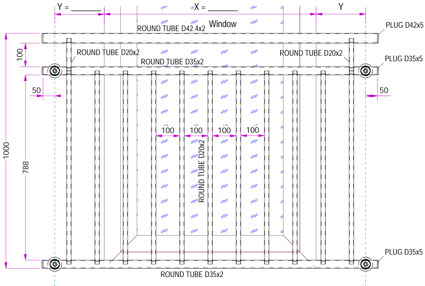
Front view 1:10
