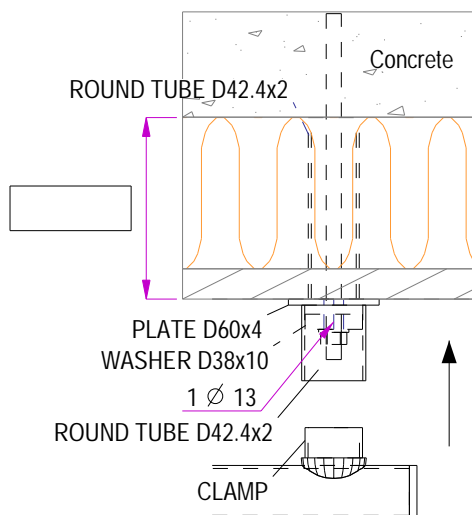
Detail 1 1:5
