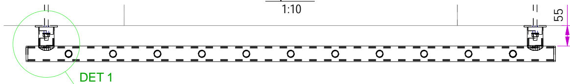
Top view 1:10
