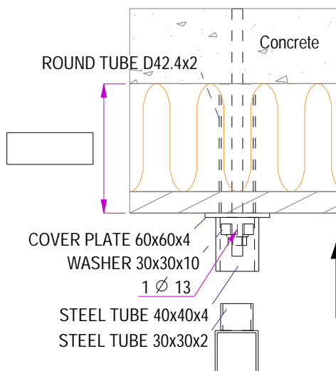
Detail 1 1:5
