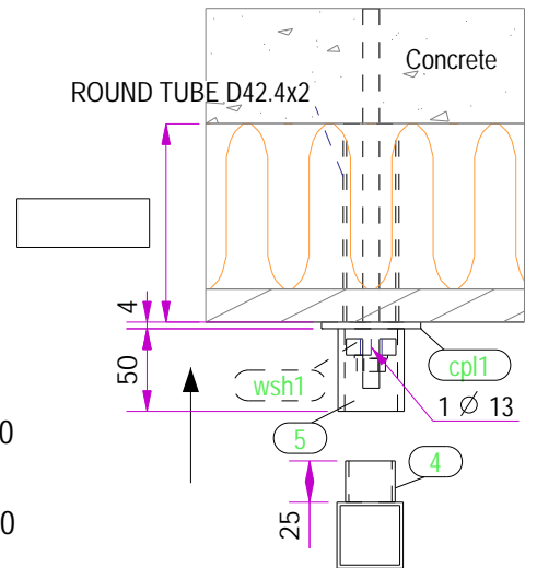
Detail 1 1:5
