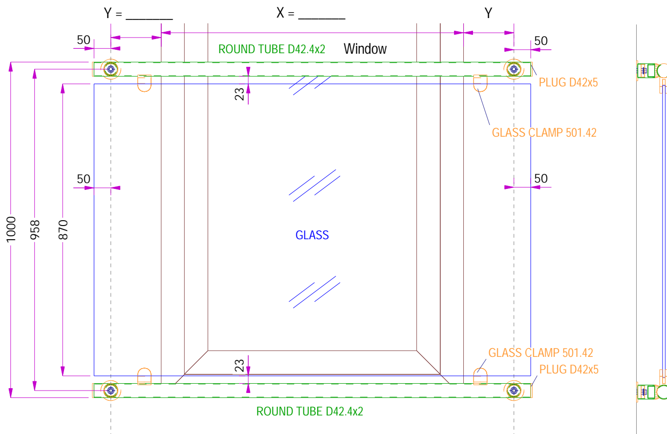
Top view
