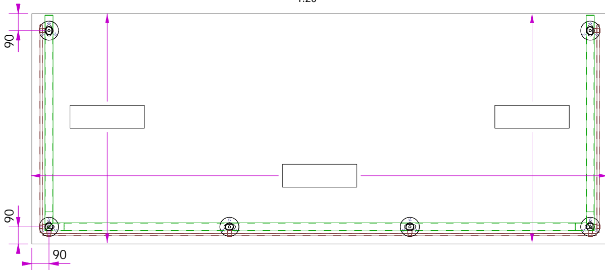
Top view 1:20
