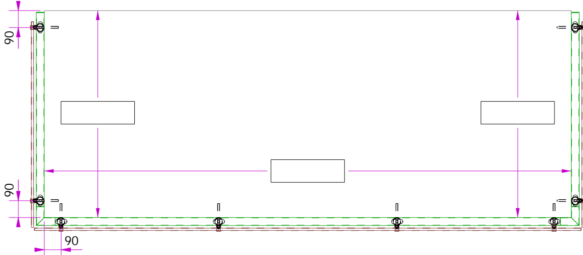
Top view 1:20
